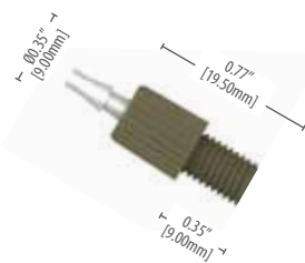
008NBxx¹-KT Series Click-N-Seal Ultra™ Thread to Barb
