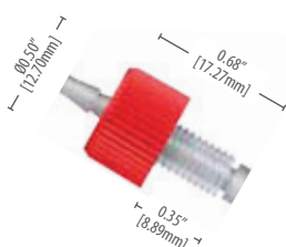
008NBxx¹-CS Series Click-N-Seal™ Thread to Barb
