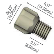
002122S PEEK™ nut for 1/16" OD tubing 1/4-28, natural
