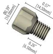
002222S PEEK™ nut for 1/8" OD tubing, 1/4•28
